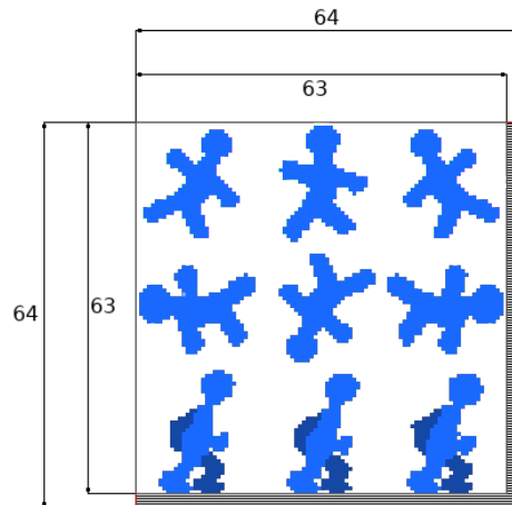
Figure 246: Example spritesheet that gets padded to match hardware constraints
